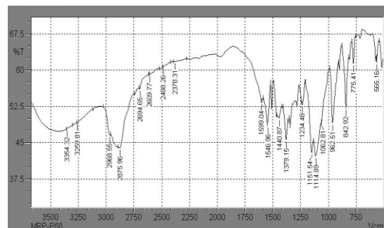
Figure 2: FTIR spectra of physical mixture
